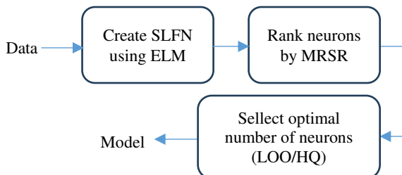
Fig. 2. OPELM algorithm stages
