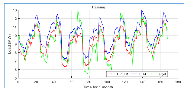
Figure 4. Plot Comparison of the Results of the Electrical Load Forecasting Training for the Next Week
