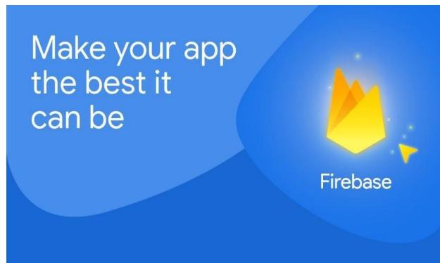
Figure 4. Firebase Software
