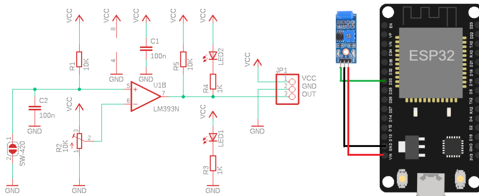
Figure 8. Vibration Sensor Module and Configuration with ESP32 Module
