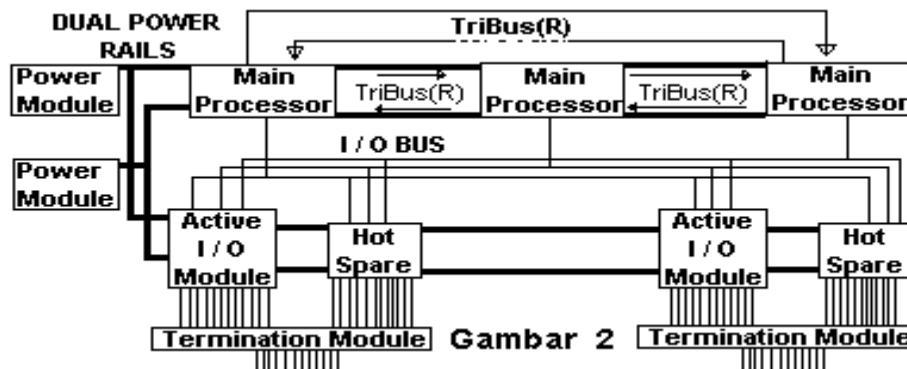
Figure 2. Interaction between module in a Trisen TS3000 PLC .
