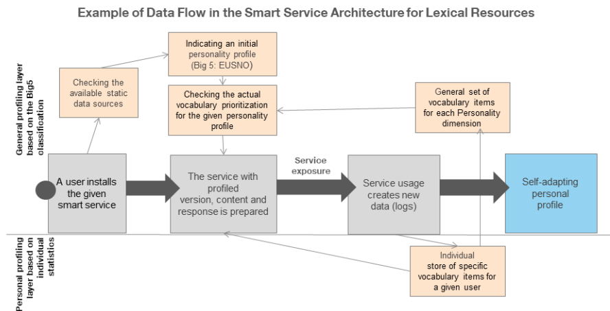
Fig. 5. Example of Data Flow in the Smart Service Architecture for Lexical Resources
