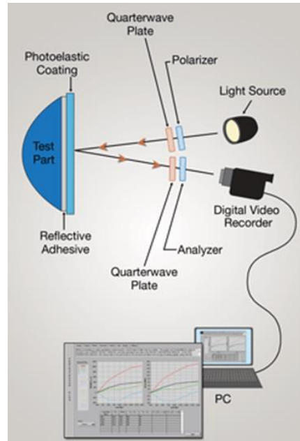
Fig. 5. System configuration.
