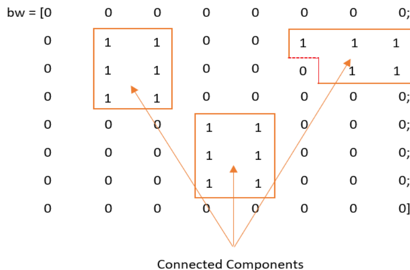
Fig.5: 3 linked components of Binary image (from [3]).
