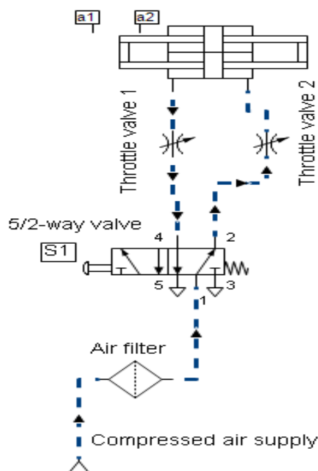
Figure 4. Simulation of the first pneumatic circuit. Simulation
