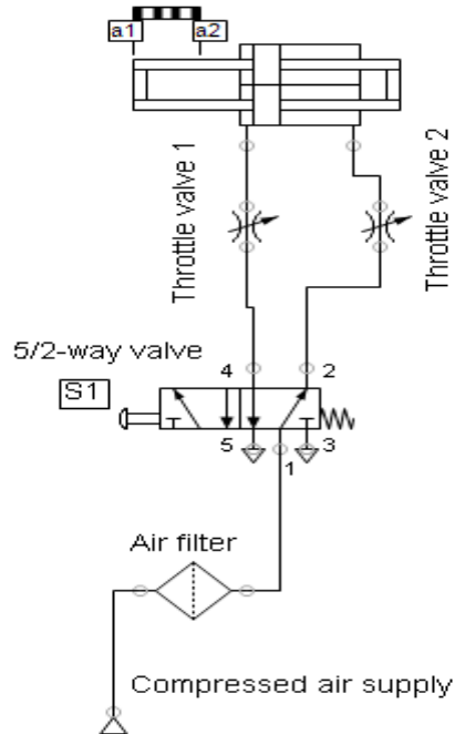
Cylinder with two in and out piston rods 1-1
