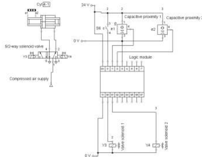
Figure 11. Second electro-pneumatic circuit using a logic module
