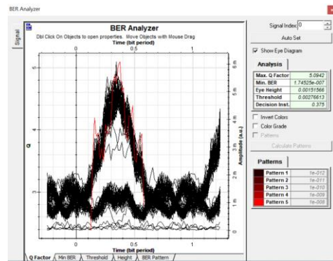
Eye diagram 1550nm wave length for 100 km cable
