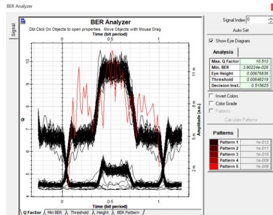
Eye diagram 1625nm wave length in 80 km cable
