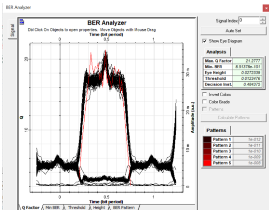
Eye diagram 1625nm wave length in 60 km cable
