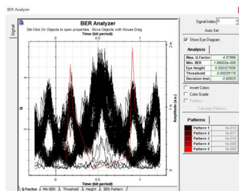
Eye diagram 1550nm wave length for 140 km cable
