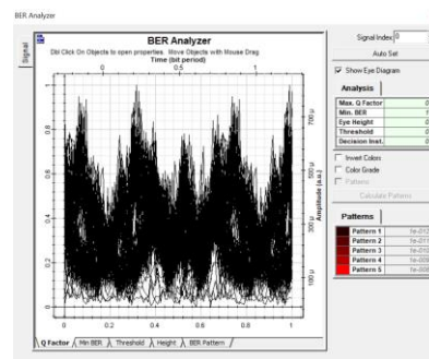
eye diagram 810nm wave length for 140 km
