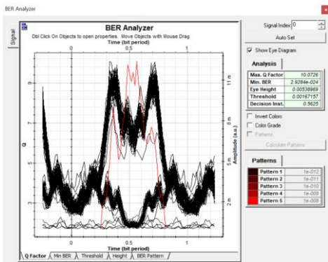
Eye diagram 810nm wave length for 80 km cable
